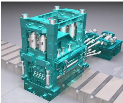
fig. 3. Cold/Hot Plate Leveler
