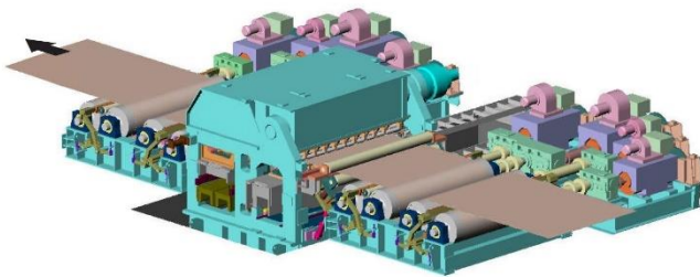
fig. 2. Tension Leveler for Advanced High Strength Steel
